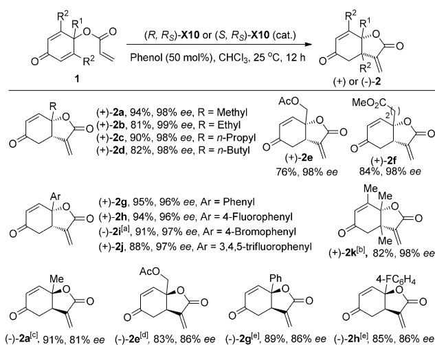
Scheme 3. The scope of the X10 -catalyzed enantioselective intramolecular Rauhut–Currier reaction. [a] 18 h. [b] ( R,R S )- X10 (20 mol%), without phenol, 72 h. [c] ( S,S S )- X10 (20 mol%), without phenol, 72 h. [d] ( S,R S )- X10 (20 mol%), without phenol, 36 h. [e] ( S,R S )- X10 (20 mol%), without phenol, 24 h.
